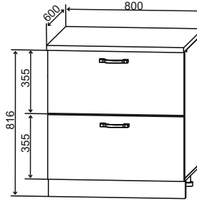
СК2 800 800/816/600
