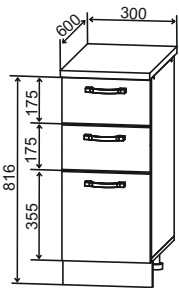
СЯШ 300 300/816/600
