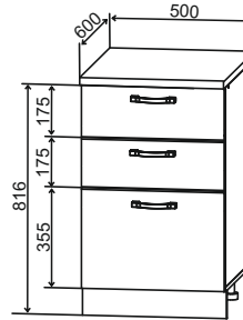
СЯШ 500 500/816/600
