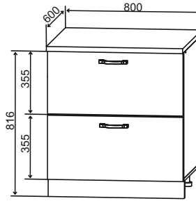
CK2 800 800/816/600
