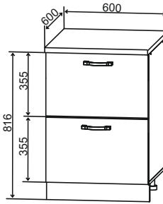
CK2 600 600/816/600
