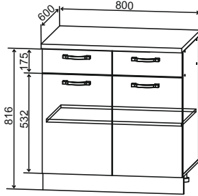
С2YШ 800 800/816/600
