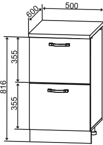
CK2 500 500/816/600
