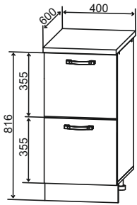
CK2 400 400/816/600
